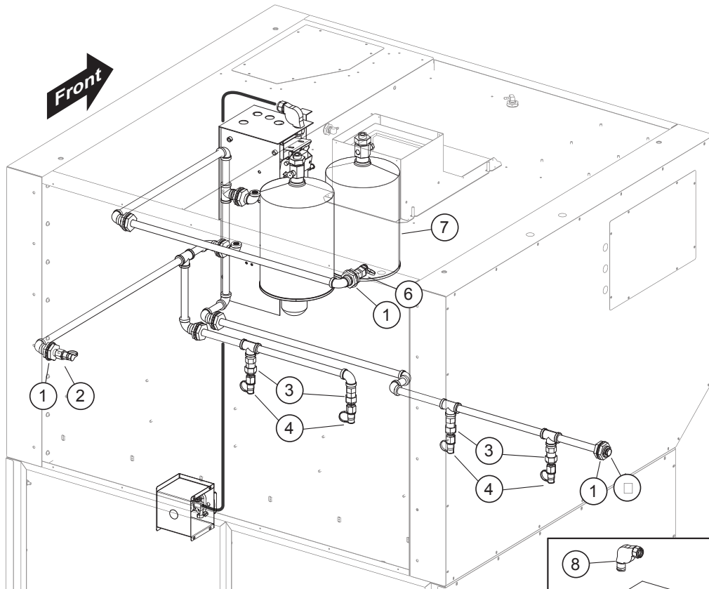
Suppression System
